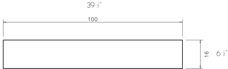
FRONTAL / FRONT
