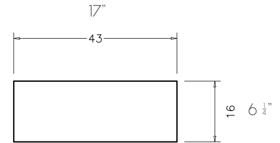
LATERAL / SIDE
